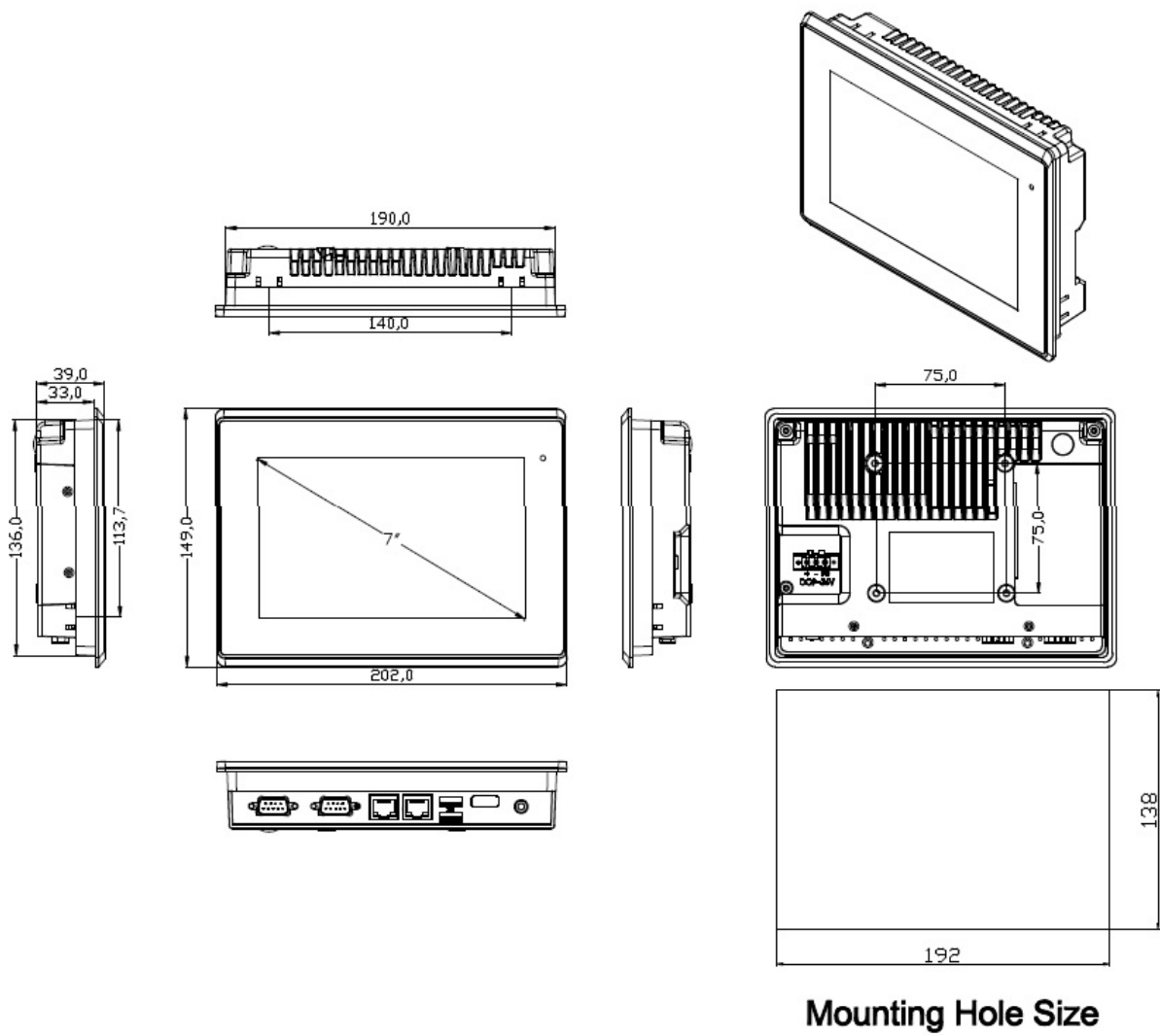
Figure 1.1: Dimensions of VISION-507
