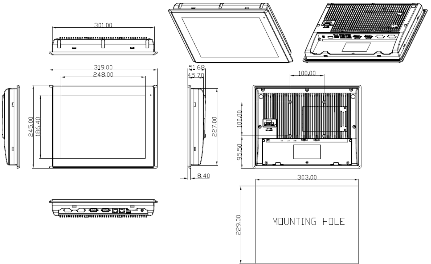
Figure 1.3: Dimensions of VISION-512
