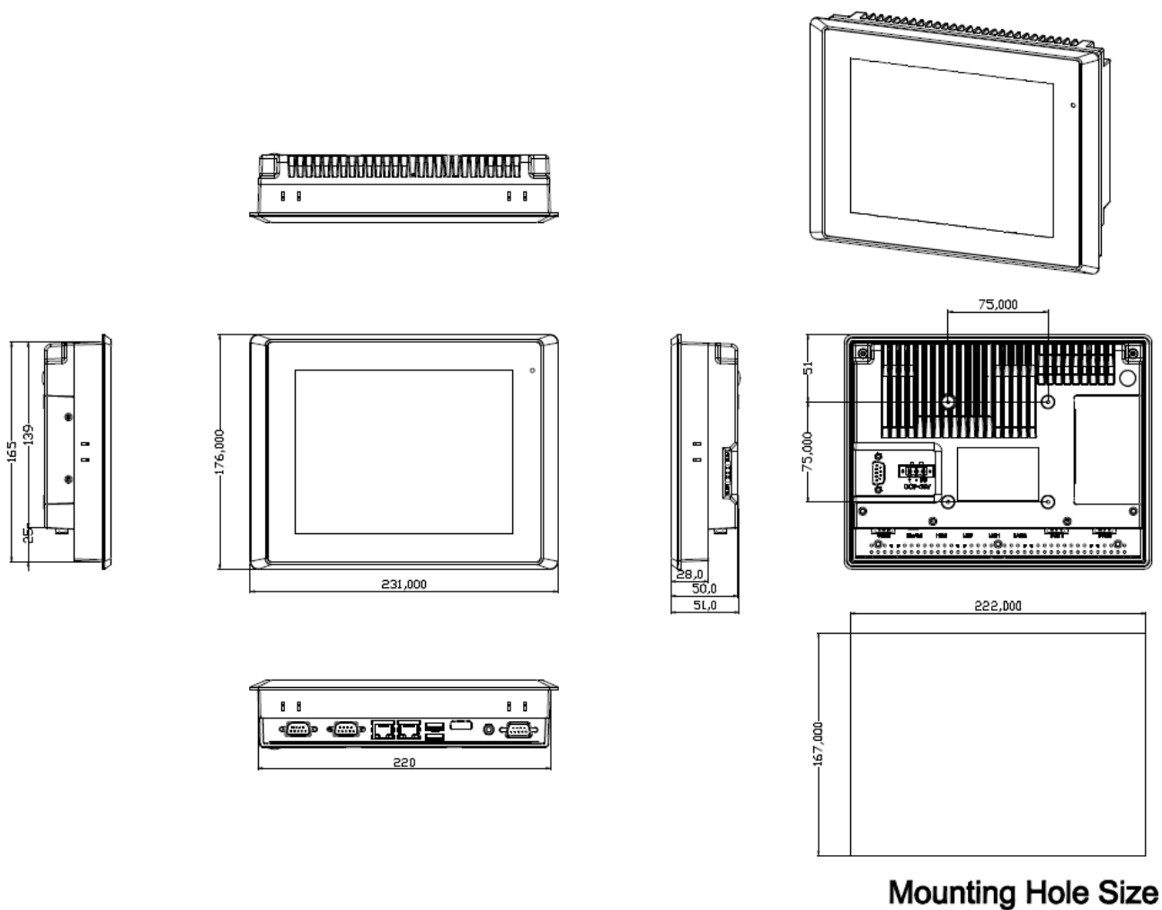
Figure 1.2: Dimensions of VISION-508
